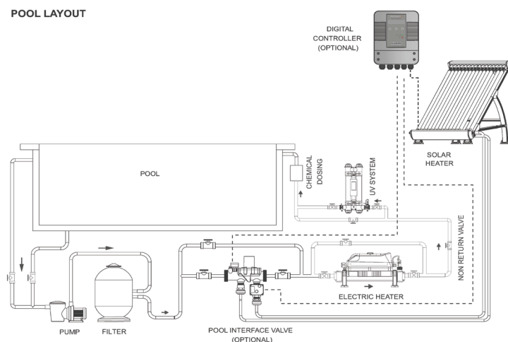
POOL LAYOUT
